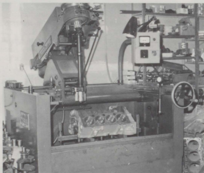
CK-10 Sunnen Boring Machine
