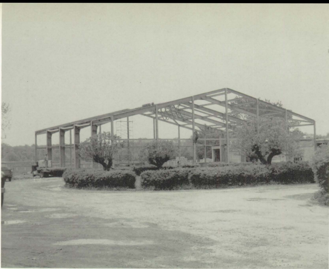
The steel skeleton is erected.
